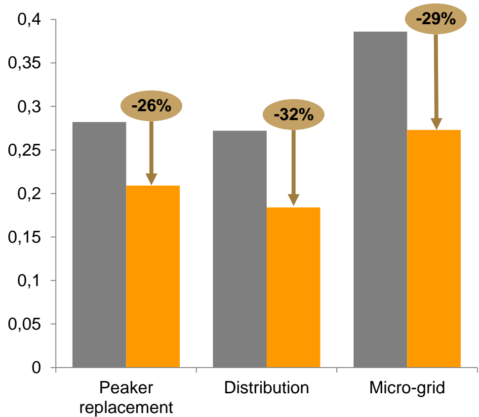
USD / kWh, 1 2017, levelised costs ■ Lithium-Ion ■ VRFB
