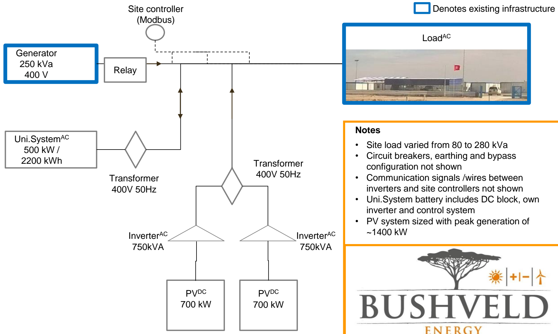
Single Line Diagram of proposed technical configuration
